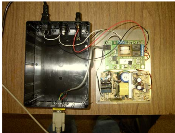
Control Box
